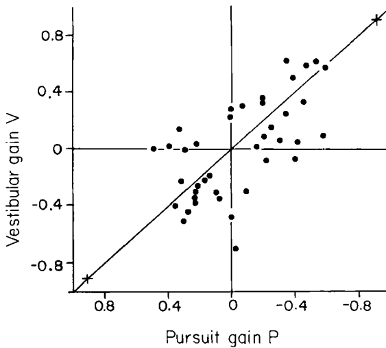
Figure 2: Plot of vestibular (V) versus pursuit (P) gains of hidden and output units in a 40 hidden unit, vestibular-pursuit neural network model. Because correctly wired units would have vestibular and pursuit gains of opposite signs, the polarity of the P axis is reversed for illustrative purposes. Hidden units (filled circles) falling on or near the horizontal or vertical axis can be considered as pure-pursuit or pure-vestibular units, respectively. The output units (+), having equal and opposite V and P values (by design), lie along the diagonal line. Hidden units falling on or near this line also have V and P values that are approximately equal and opposite. Most units are scattered throughout quadrants 1 and 3 and, having V and P of opposite sign, encode eye movements in the same direction. However, a small percentage of hidden units fall in quadrants 2 and 4 and have V and P of the same sign. Such seemingly anomalous units have been occasionally observed experimentally (Chubb et al. 1984; Fuchs and Kimm 1975; Miles 1974; Tomlinson and Robinson 1984).
