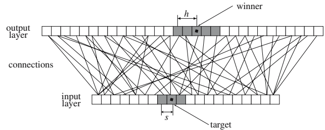
Fig. 1 The one-dimensional SOM network. Input units (bottom) are connected to output units (top) via synaptic weights. Locations of the target and the winning output unit are marked with a black square. The shaded units in the input layer are driven by the target; the remaining input units fire spontaneously. The shaded units in the output layer are contained in the neighborhood of the winner. Also shown are the spatial tuning s (here equal to 1) and the neighborhood size h (here equal to 2)
