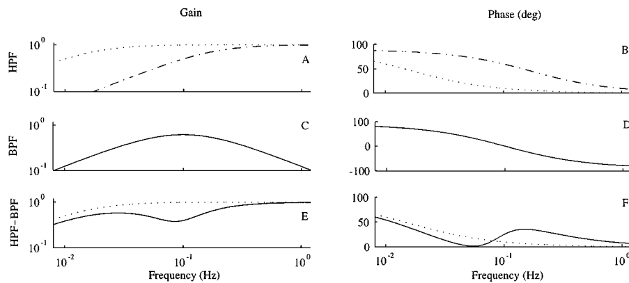
Figure 1. Prototypical frequency responses from the HPF-BPF model (Fig. 5). A, B: The naïve VOR frequency response (dotted lines) was modeled as a first-order HPF. For comparison, modeling habituation by decreasing the time constant of a that HPF by an order of magnitude is shown by the dot-dashed lines. C, D: The frequency response of a BPF. E, F: The difference (HPF-BPF, solid line) shows the gain dip and phase crossover not seen in the naïve HPF (dotted lines). The gain constant of each transfer function is identical ( g_v = g_b = 1 ). Values of other parameters are \tau_v = 10.4 s, cf = 0.1 Hz, and \lambda = 0.1 ( \tau_l = 1.26 s and \tau_h = 2.00 s). The subtraction causes a decrease in gain centered on the cf and also causes a decrease in phase lead at nearby lower frequencies and an increase in phase lead at nearby higher frequencies. The resultant dip in gain is shifted to lower frequency, as is the phase crossover, due to the phase lead and gain decrement of the HPF.
