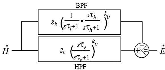
Figure 5. Schematic diagram of the combined HPF-BPF VOR model. The model converts head velocity ( \dot{H} ) to eye velocity ( \dot{E} ). The values used for the naïve goldfish HPF were: \tau_v = 10.4 s and k_v = 0.23 . The gain constant of the HPF ( g_v ) was adjusted to match the highest gain value in the habituated data. The gain constant for the BPF ( g_b ) was fixed at 0.3 and the order ( k_b ) was fixed at 1.0. The time constants for the low- ( \tau_l ) and high- ( \tau_h ) pass filters that defined the BPF were determined separately for each frequency of habituation (see Results) using a least-squares optimization routine and are shown in Table 1.
