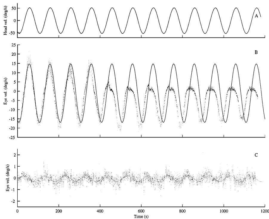
Figure 2. Time series illustrating the habituating and habituated VOR at 0.01 Hz. Inverted head velocity during 0.01 Hz rotations (A) is compared to the VOR eye velocity of naïve habituating (B) and habituated (C) goldfish. To show changes in VOR gain and phase the sinusoids shown in (B) and (C) were fit by minimizing the least-squares error for the first cycle of the data only and then propagated with the same parameters to the end of the graph. Phase lead increases during the first 20 min of 0.01 Hz rotation (B) and becomes pronounced during the fifth cycle. The VOR eye velocity waveform also becomes distorted during the fifth cycle (nasal rectification), though nonsinusoidal portions are observable on the second cycle. C: Habituation becomes severe after 40 min of rotation. The response is attenuated but clearly sinusoidal. The vertical scales for (B) and (C) are different. Nasally and temporally directed eye rotational velocities are given positive and negative values, respectively.
